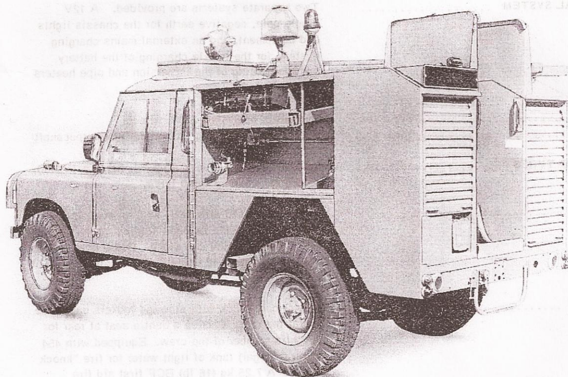
TRUCK, FIREFIGHTING, Airfield crash rescue, 1 ton, 4 x 4, Rover
